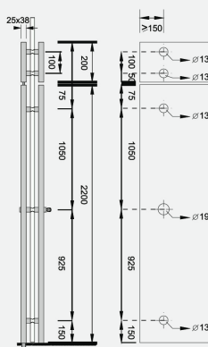
CORTE DE CRISTAL DR8200D-6 / DR8200D-6A
